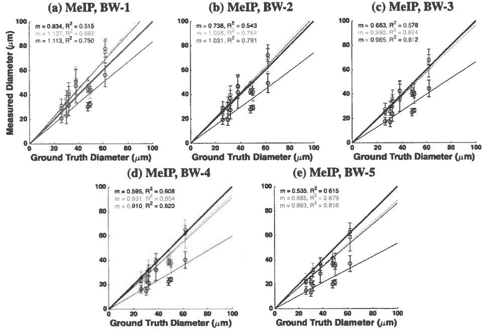
Fig. 6. Vessel diameter measured from binarised masks versus ground truth for MeIP at five threshold levels: (a) BW-1 through (e) BW-5. Linear regression lines and statistics are shown for pre-contrast (blue), peak contrast (green), and post-contrast (red) conditions.
